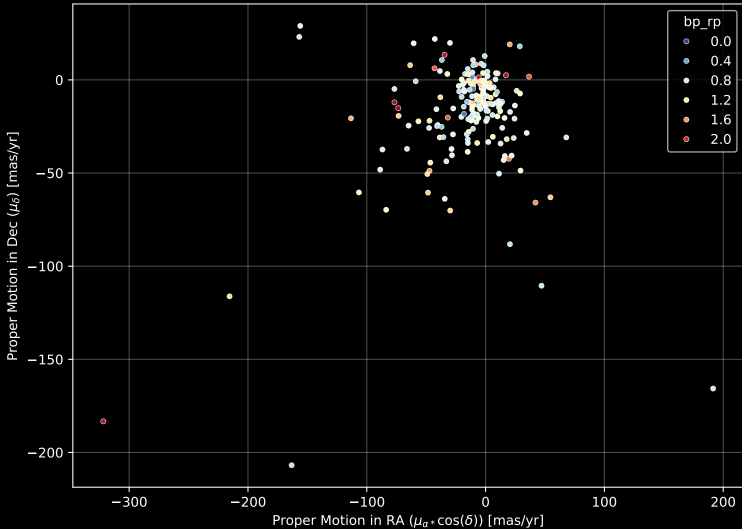
APOGEE DR17 Field: [191+50_MGA] Proper Motion Diagram (n= 198)
