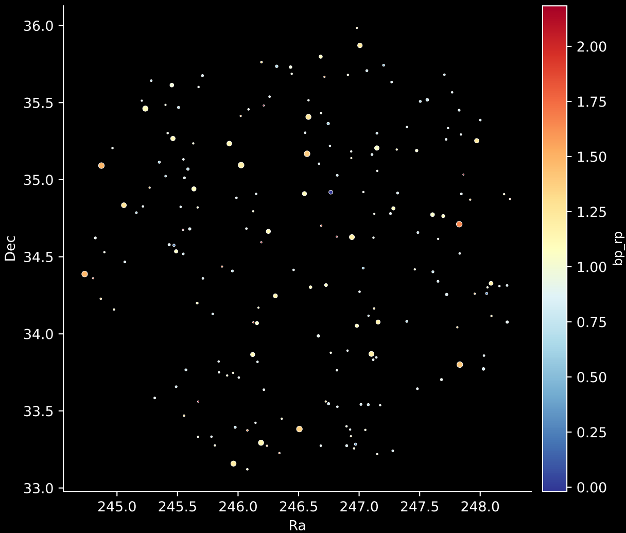
APOGEE DR17 Field: [191+50_MGA] Stars: 198
