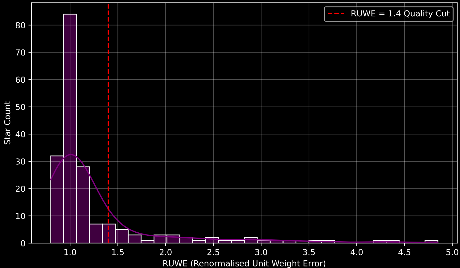
GAPOGEE DR17 Field [191+50_MGA] RUWE Distribution (n= 190)
