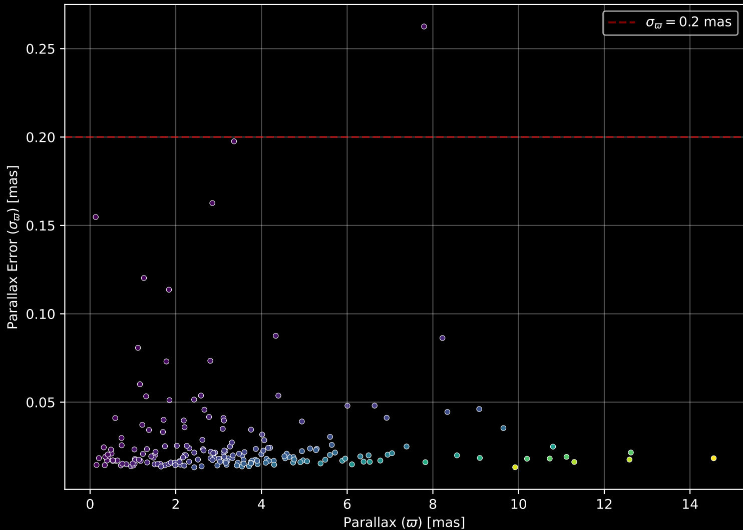
APOGEE DR17 Field: [191+50_MGA] Parallax Quality (n= 198)
