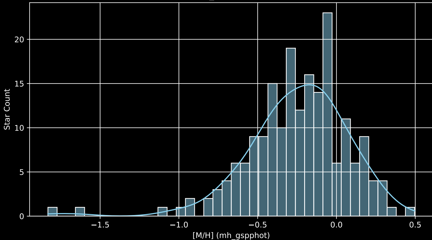
APOGEE DR17 Field: [191+50_MGA [M/H] (mh_gspphot) (n= 196)
