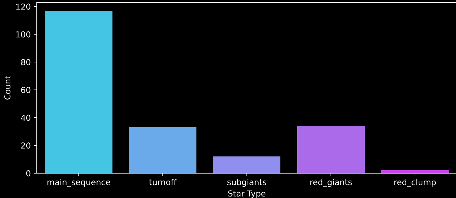
APOGEE DR17 Field: [191+50_MGA] Count plot of Star Type
